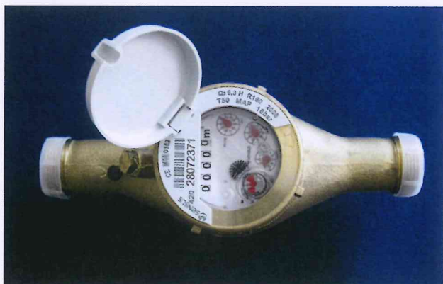
Picture No. 8 Multi jet meter 420/PC Q 3 6,3 inline (top view and side view)
