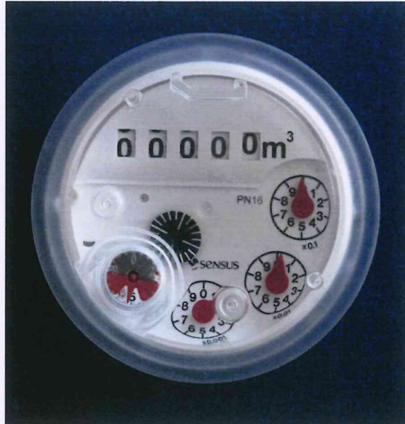
Picture No. 15 Register 420 Q 3,2,5 – 16 with the possibility of HRI adaption
