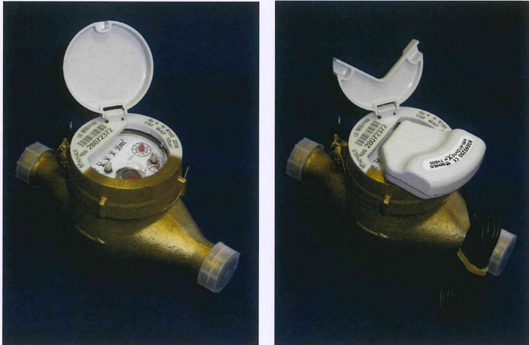
Picture No.5 Multi jet meter 420/PC Q 3 4 inline without and with HRI (perspective view)
