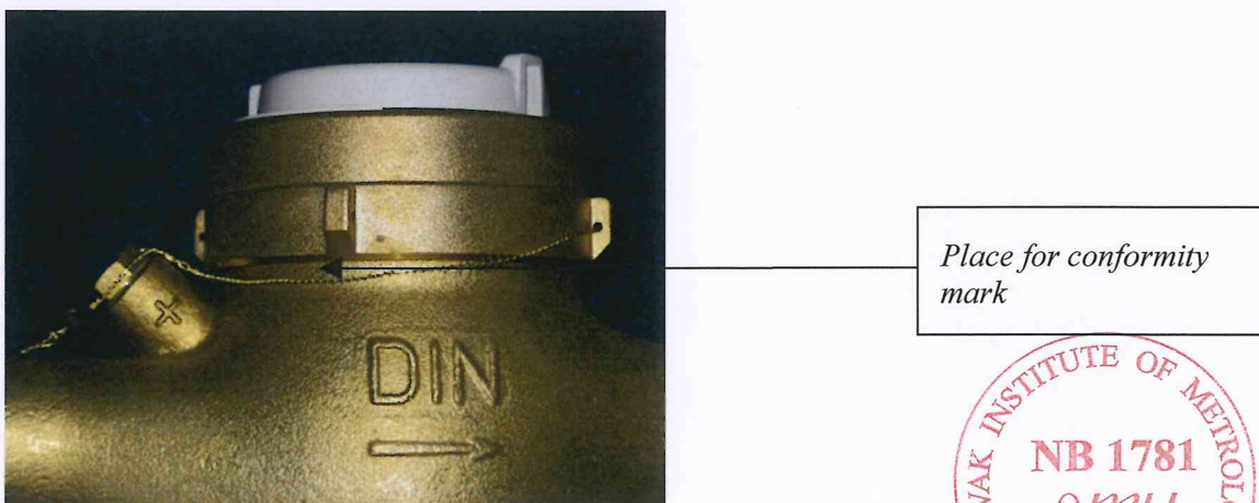
Picture No. 18 Sealing with a long loop - inline -
